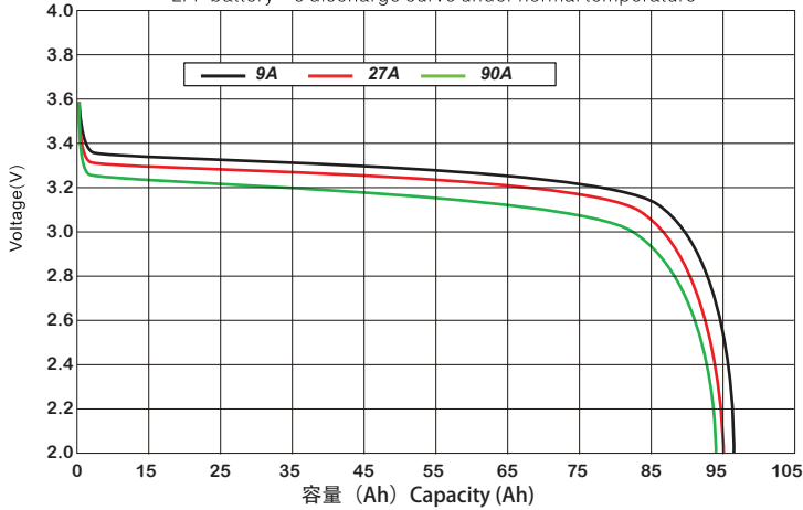
常温下 LFP类电池的放电特性曲线 LFP battery's discharge curve under normal temperature
