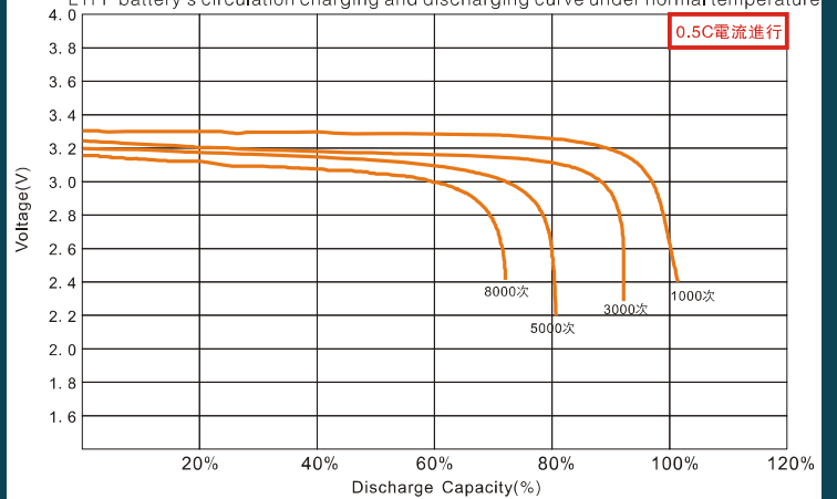
常溫下LYP類電池的循環充放電特性曲線 LYFP battery's circulation charging and discharging curve under normal temperature
